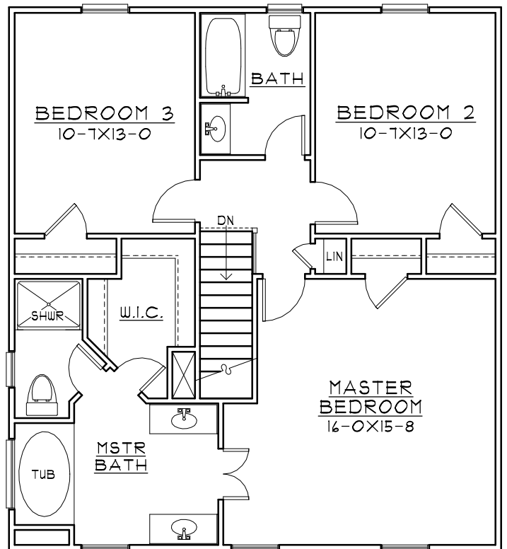
SECOND FLOOR PLAN 928 SQ. FT.
