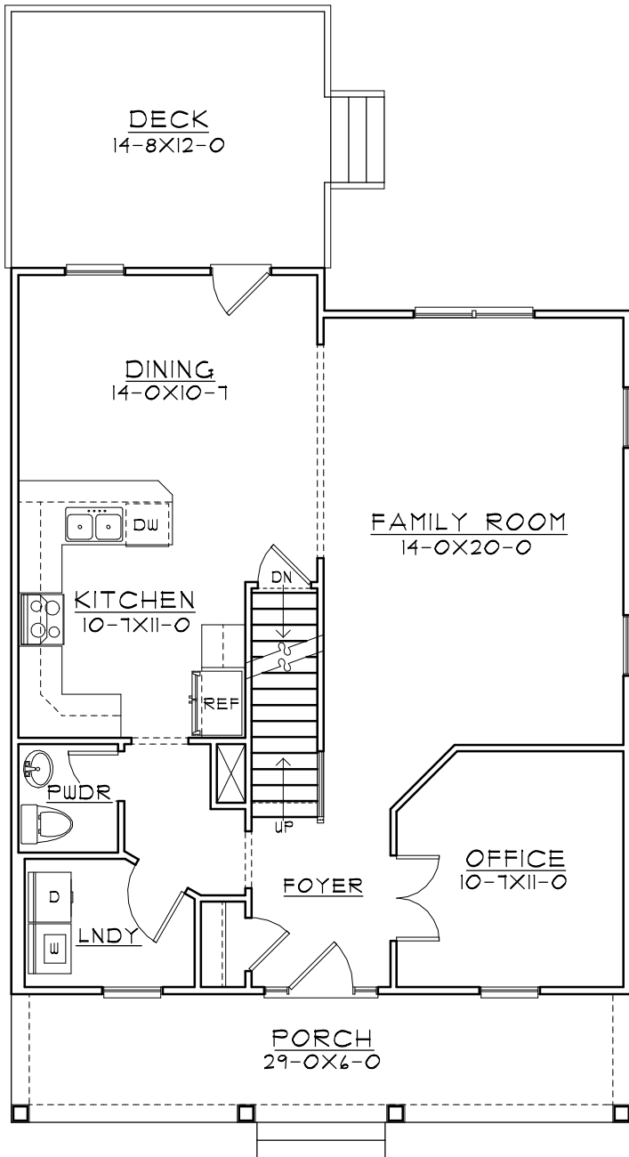
FIRST FLOOR PLAN 957 SQ. FT.
